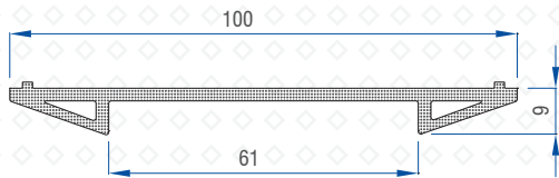
Casement Sliding Middle Coupler 2.5T (I-64) 50502 - 11063
