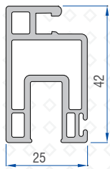
Screen Sash Profile 41301-05200
