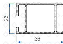
Multi Track Adaptor(Alm) 50502-11017
