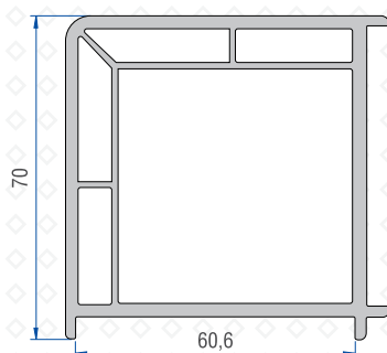
Corner Profile (90°) 40104 - 02000
