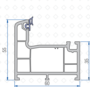
Frame Profile 41101 - 11000
