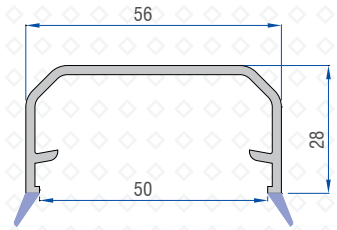
Hurricane Bar Profile 40201-01000
