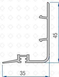
Sash Cover Profile 41201 - 06100
