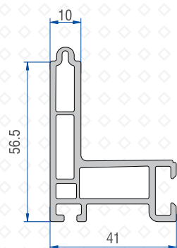
Screen Sash Adaptor 41321 - 05300
