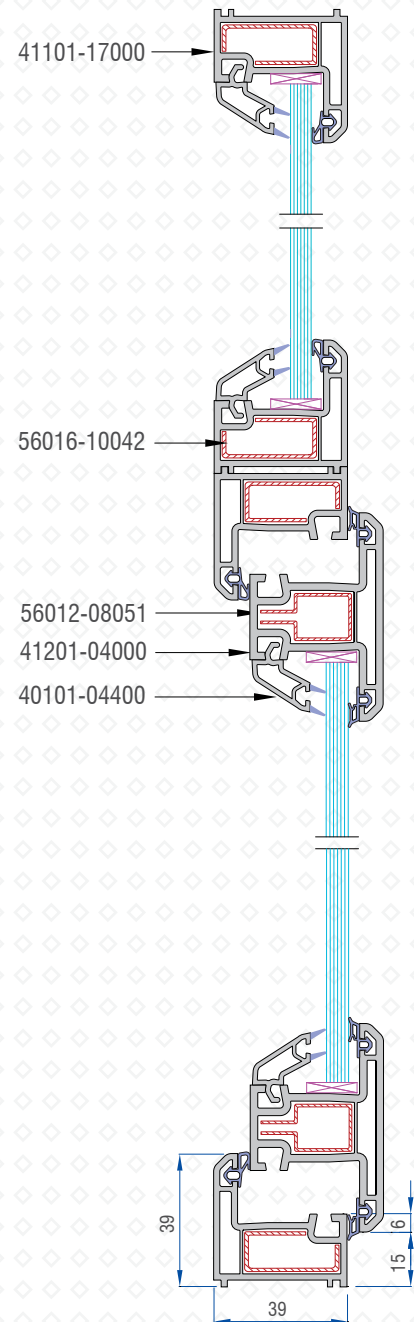
SEC B-B
