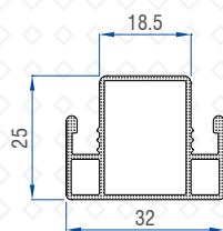
Screen Sash Mullion (Alm) 50502-11037
