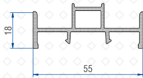
Inline Sash Adaptor (Alm) 50502 - 11035
