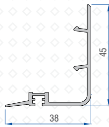
65mm Sash Cover Profile 41201 - 06200
