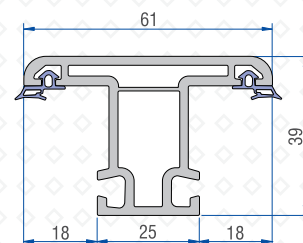
Mullion Profile 41201 - 04000
