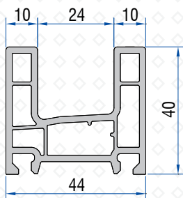
Double Rail Profile 41231-02000
