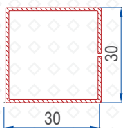
Double Rail Reinforcement 1.0mm : 56016 - 10301
