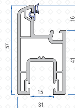
Sash Profile 40502-13000
