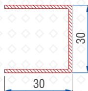
Double Rail Reinforcement 1.0mm : 56016 - 10302
