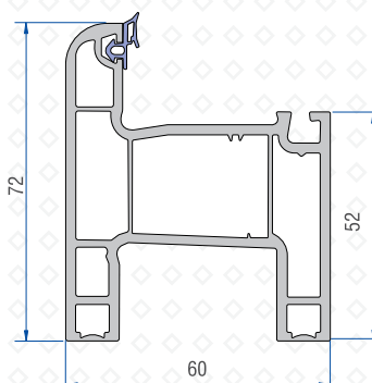
Casement - Sliding Mullion Profile 41201 - 14100
