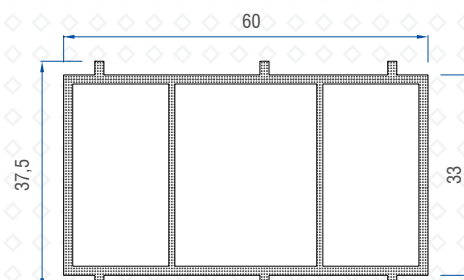
Casement Sub Frame 50502-11068
