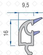
Single Glazing Bead 40502-14000
