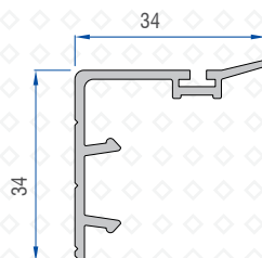
Sash Cover 40502-13100
