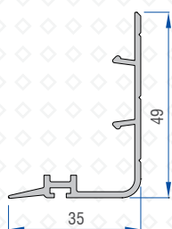
Sash Cover Profile 41064 - 40100
