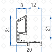
Mesh Adaptor(Alm) 50502-11055
