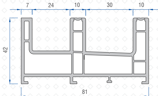
Double Rail with Screen Track Profile 40502-12000
