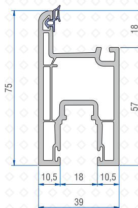
Super Sash Profile 41201 - 03000
