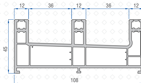
Triple Rail Profile 41201 - 05000
