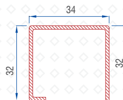
Super Sash Reinforcement 1.5 mm : 56016 - 15137
