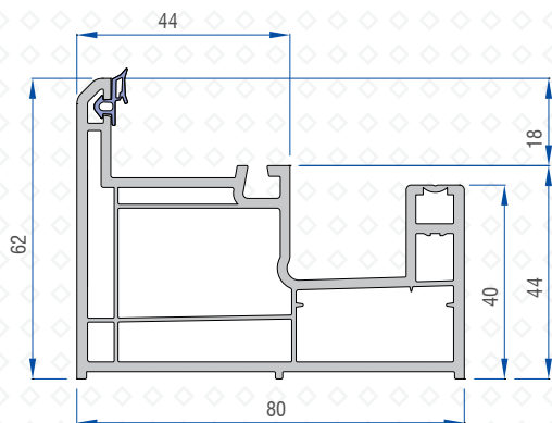
Mono Rail Profile 41164-10400
