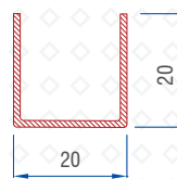
Screen Sash Reinforcement 1.5mm : 56016 - 15501
