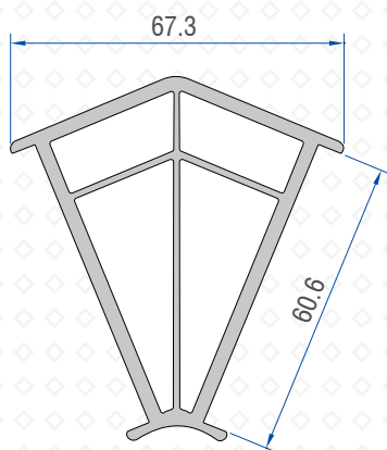
Corner Profile (135°) 40104 - 01000
