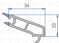
Single Glazing Bead (6mm) 40101 - 03300
