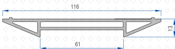
Casement Sliding Middle Coupler 3T (I-64) 50502 - 11064
