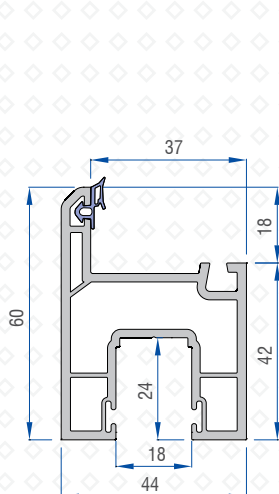
Sash Profile 41164-20100
