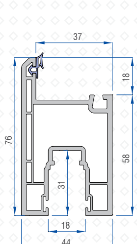
Super Sash Profile 41164-20300
