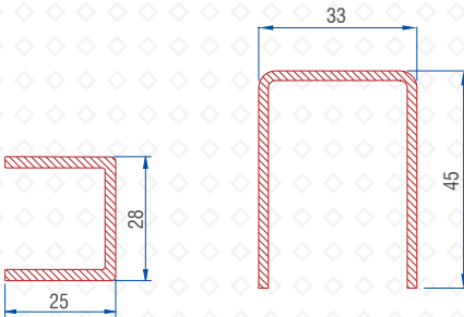
Super Sash Reinforcement 1.5 mm : 56016 - 15017
