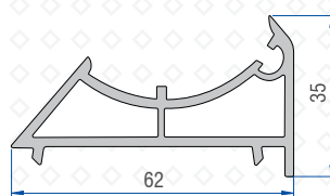
Pipe Adaptor Profile 40104 - 03100
