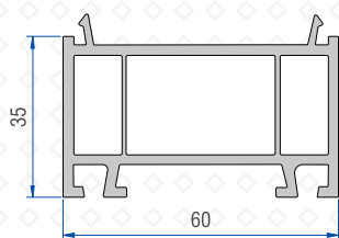
Frame Lifting Profile 40106 - 02100
