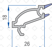
Single Glazing Bead (6mm) 41064-30100
