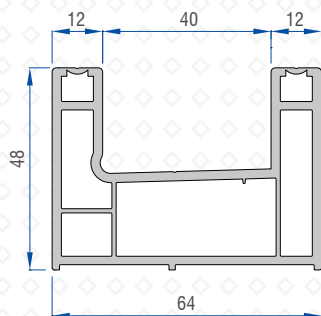
Double Rail Profile 41164-10100
