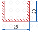
Frame / Mullion Reinforcement 1.0mm : 56016 - 10002
