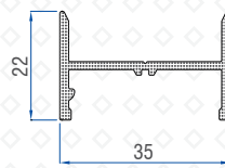
Adaptor for Super Screen Sash 50502 - 11049
