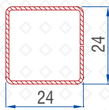
Mullion Reinforcement 1.0mm : 56016 - 10044
