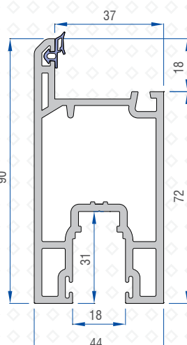
Mega Sash Profile 41264-20400
