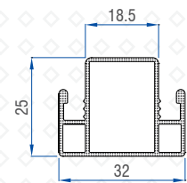
Screen Sash Mullion(Alm) 50502-11037
