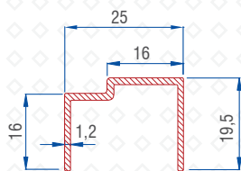
I-50 Sash Reinforcement 56016 - 12107
