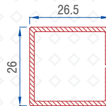
Mega Sash Reinforcement(Secondary) 1.5mm : 56016 - 15057
