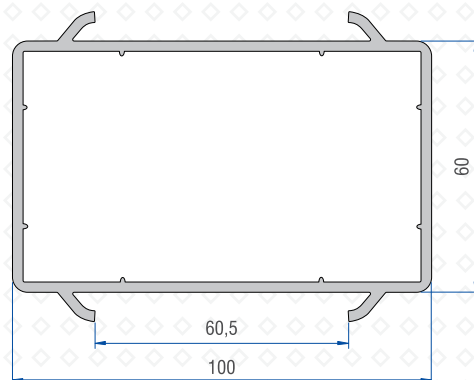
Box Profile (60 x 100) 40107 - 01100
