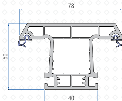
Mullion Profile 41221 - 13000
