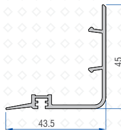
Super Sash Cover Profile 41201 - 06000
