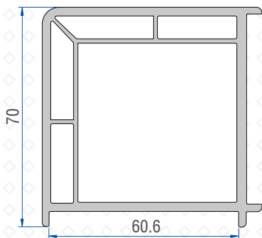
Corner Profile (90°) 40104 - 02000
