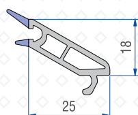
Single Glazing Bead (6mm) 40101 - 04300
