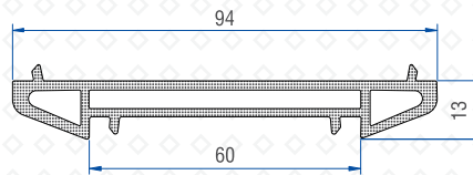
Casement - Sliding Profile Middle Couple (Alm) 50502 - 11040
