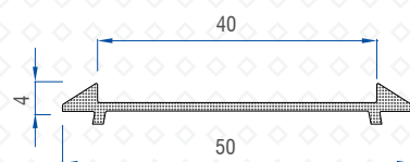
Frame Coupler I-50(2T) to I-39 50502-11066
