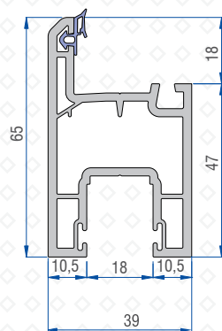
65mm Sash Profile 41201 - 03200
