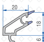
Single Glazing Bead (6mm) 40101 - 04400
