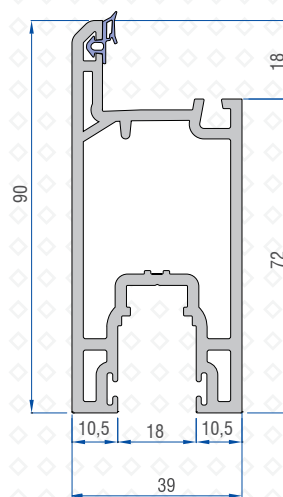
Mega Sash Profile 41201 - 07000
