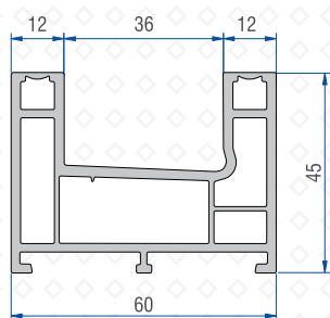
Double Rail Profile 41201 - 02000
