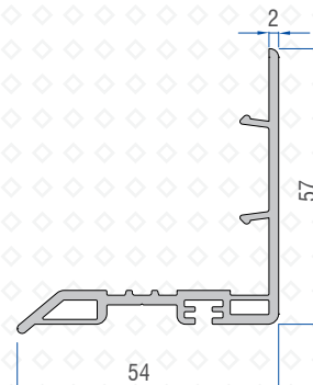
Mega Sash Cover Profile (New) 41221 - 07100
