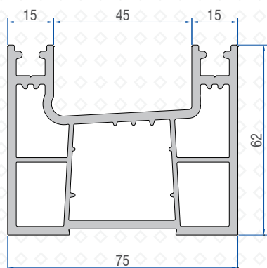
Double Rail Profile 41221 - 01000
