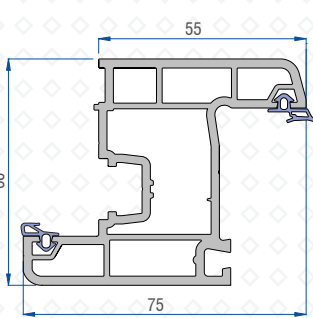
Inward Opening Sash Profile 41101-13100
