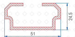
Hurricane Bar Reinforcement 2.0 mm : 56016 - 20020
