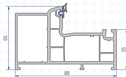
Frame with Grill 41101 - 16000
