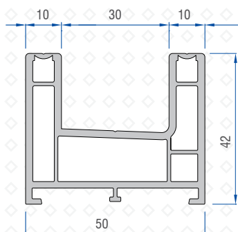
Double Rail Profile 40502-11000
