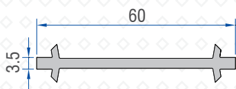
COUPLING PROFILE 40107 - 01400
