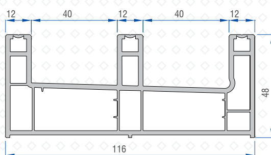
Triple Rail Profile 41164-10300
