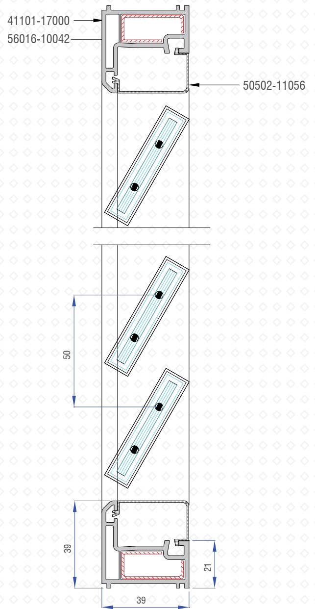
SEC B-B
