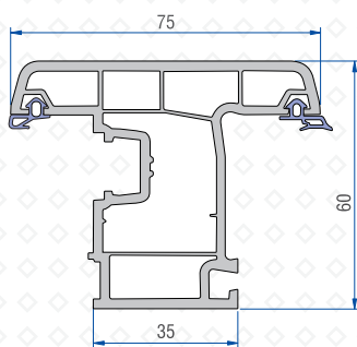
Window Sash Profile 41101 - 13000
