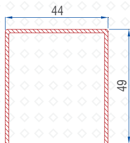
Sash Reinforcement 1.5mm : 56016 - 15311
