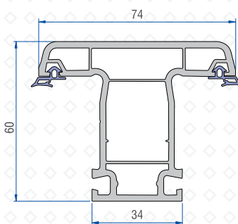
Mullion Profile 41101 - 12000
