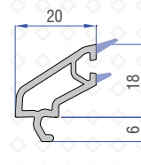
Single Glazing Bead (6mm) 40101-04400
