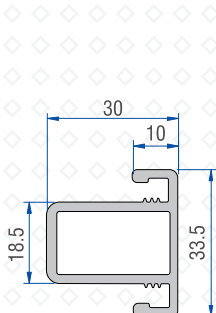
Sash Profile 41221 - 12000
