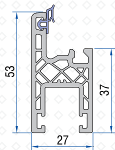
Sliding Sash 41231-13100
