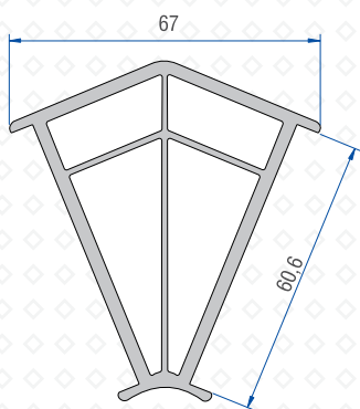
Corner Profile (135°) 40104 - 01000
