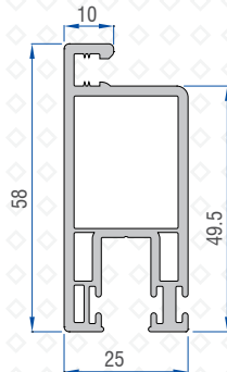
Mega Screen Sash Profile 41201 - 05300
