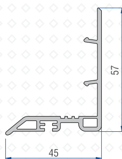
Sash Cover Profile 41221 - 06100
