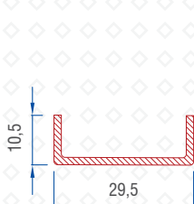
2T/2.5T Frame Reinforcement 56016 - 10007
