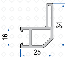
Screen Sash Adaptor 41301-05100
