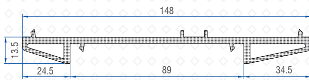
Coupler for Mesh and Grill Frame (Alm) 50502 - 11046
