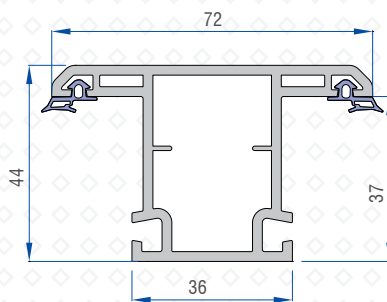
Mullion Profile 41164-20500
