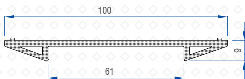
Casement Sliding Middle Coupler 2.5T (I-64) 50502 - 11063
