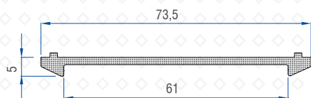
Frame Coupler I-60 Monorail to I-60 50502-11067
