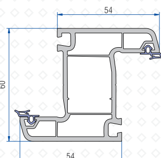
Outward Opening Mullion Profile 41101 - 12100
