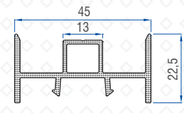
Inline Sash Adaptor (Alm) 50502-11060
