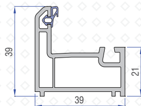
Compact Frame Profile 41101-17000
