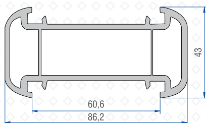
Large Coupling Profile 40107 - 01200
