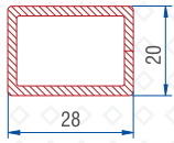
Frame / Mullion Reinforcement 1.0mm : 56016 - 10001
