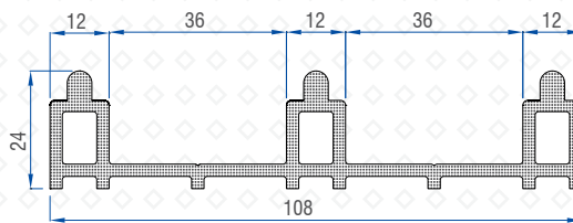
3-Track Low Threshold(Alm) 50502-11047
