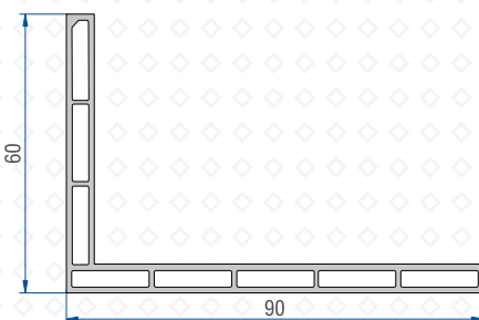
Border Profile 40110 - 02000
