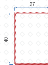
Large Frame Reinforcement 1.0mm : 56016-10056
