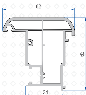
Lap Joint Profile 41101 - 15000
