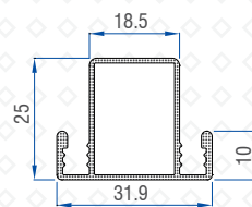
Mega Screen Sash Mullion-2.5T (Alm) 50502-11058
