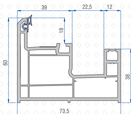
Mono Rail Profile 41201 - 08000
