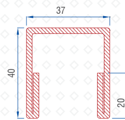
Mega Sash Reinforcement 1.5 mm : 56016 - 15147
