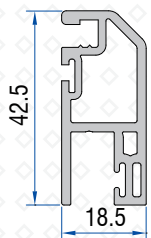
Adaptor Screen Sash 41301-05000
