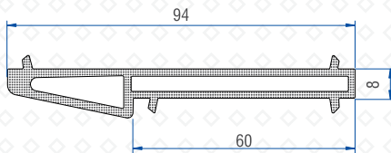
Casement - Sliding Profile Couple (Alm) 50502 - 11039
