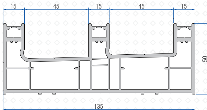
Triple Rail Profile 41221 - 02000
