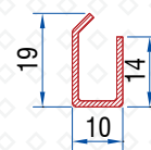
Adaptor Screen Sash Reinforcement 1.2mm : 56016 - 12041
