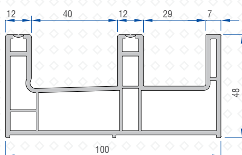
Double Rail with Screen Track Profile 41164-10200
