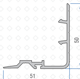
Mega Sash Cover Profile 41064 - 40300
