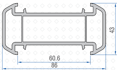
LARGE COUPLING PROFILE 40107 - 01200
