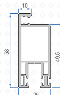
Mega Screen Sash Profile 41201 - 05300
