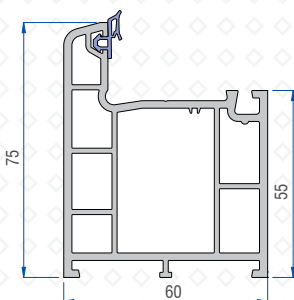
Large Frame Profile 41101-19000
