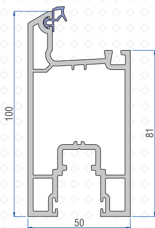
Mega Sash Profile (I-75) 41221 - 14000
