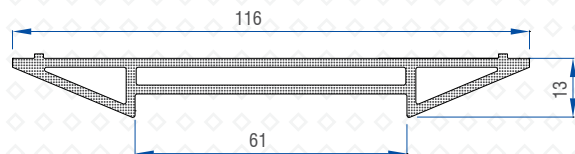
Casement Sliding Middle Coupler 3T (I-64) 50502 - 11064
