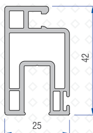
Screen Sash Profile 41301-05200
