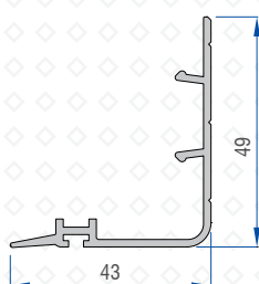
Super Sash Cover Profile 41064 - 40200
