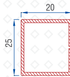
Mega Screen Sash Reinforcement 1.5mm : 56016 - 15601
