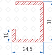
Window Sash Reinforcement 1.5mm : 56016 - 15011
