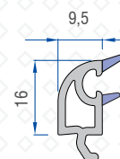
Single Glazing Bead 40502-14000
