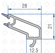
Single Glazing Bead (12mm) 40101 - 03200
