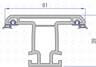
Sash/Mullion profile 41201-04000
