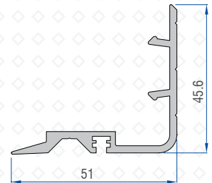
Mega Sash Cover Profile 41201 - 06300
