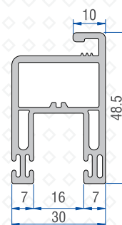
Super Screen Sash Profile 41321 - 03000
