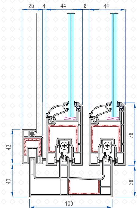
SEC B-B
