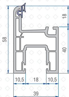
Sash Profile 41201 - 03100
