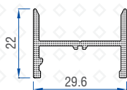
Adaptor for Screen Sash-2.5T (Alm) 50502-11048
