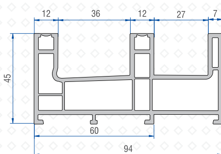
Double Rail with Screen Track Profile 41201 - 05100
