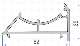
Pipe Adaptor Profile 40104 - 03100
